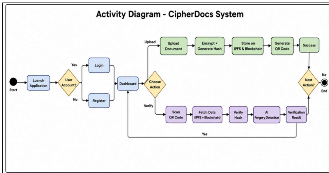
Figure 6.4. Activity Diagram — CipherDocs Document Lifecycle
