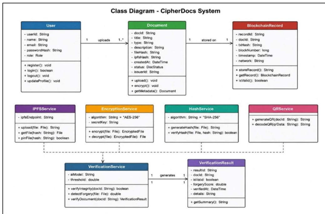
Figure 6.2. Class Diagram — CipherDocs
