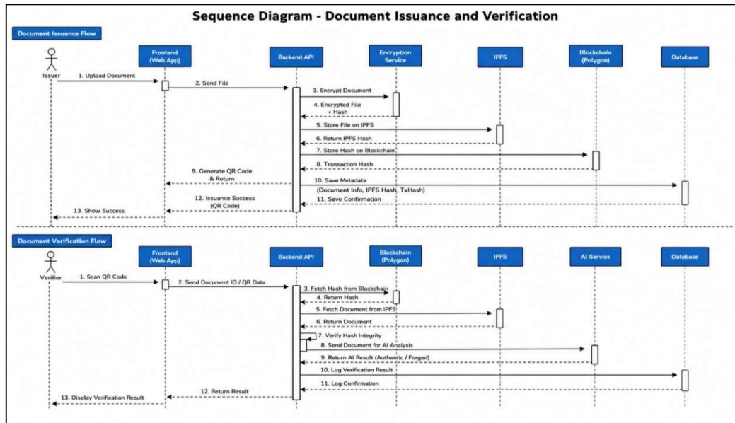
Figure 6.3. Sequence Diagram — Document Issuance and Verification Flows
