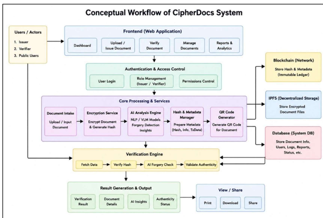
Figure 1.1. CipherDocs Conceptual Workflow
