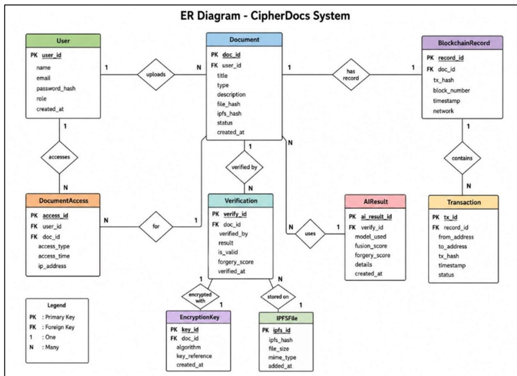
Figure 6.5. Entity-Relationship (ER) Diagram — CipherDocs
