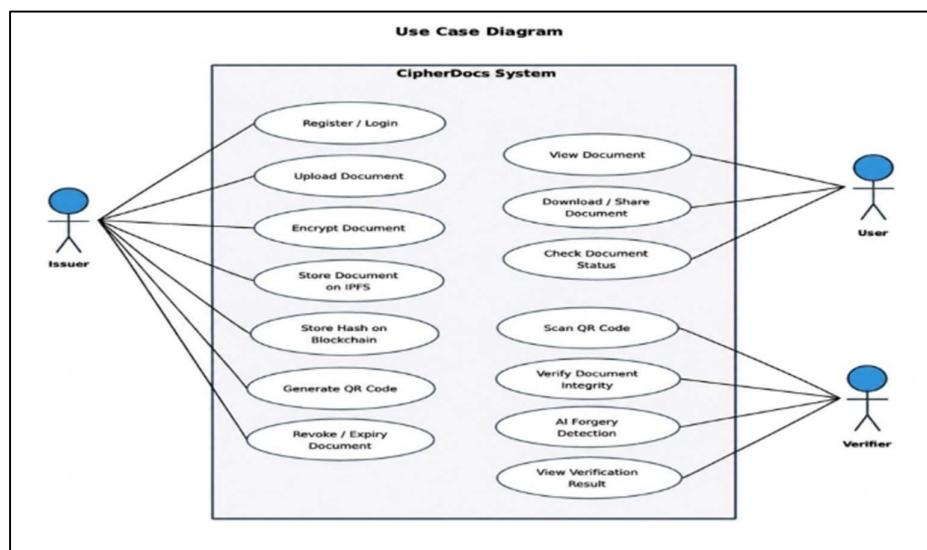
Figure 6.1. Use Case Diagram — CipherDocs
