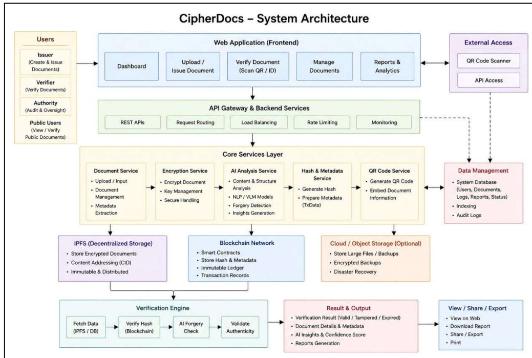
Figure 5.1. CipherDocs System Architecture
